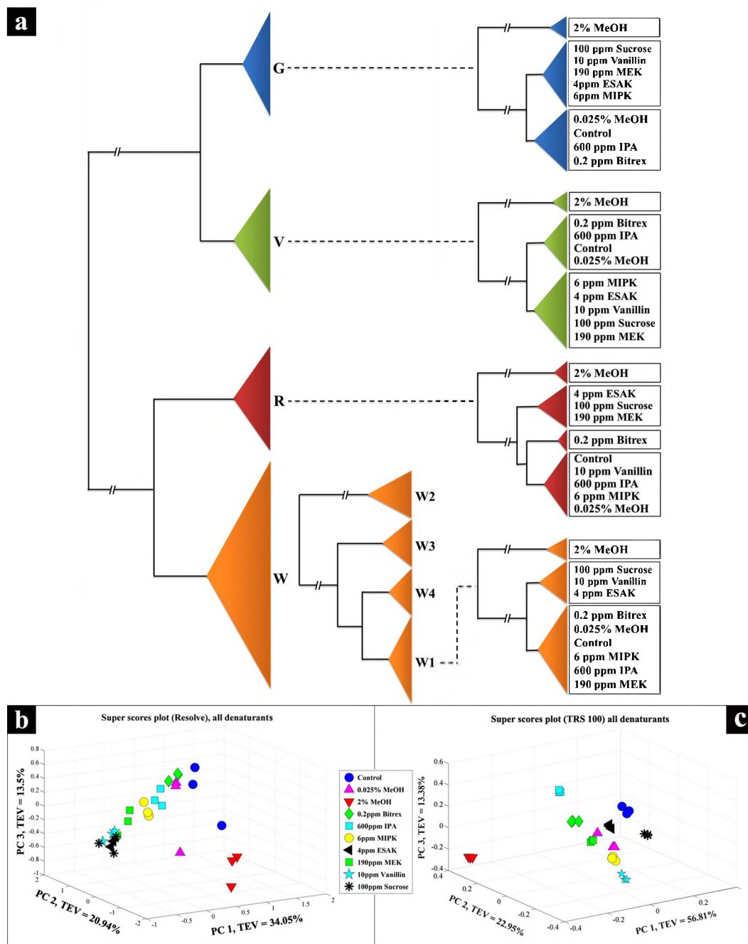
Figure 1. (a) Abridged dendrogram obtained by hierarchical cluster analysis of the PC-DFA scores of all the Raman spectral data collected using SORS; encoding used: gin (G), vodka (V) rum (R), 4 brands of whisky (W1-W4). MB-PCA super scores plots of the Raman spectral data collected using, (b) SORS with a Resolve instrument and, (c) TRS with a TRS100 instrument. Different symbols represent the different additives, and the abbreviations are shown in Table 1.
