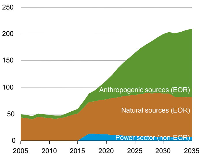
Figure 35. CO 2 injection volumes in the Reference case, 2005-2035 (million metric tons per year)
