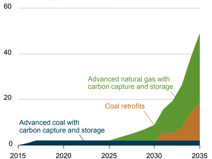
Figure 36. CCS capacity additions in the U.S. electric power sector in the GHG Price Economywide case, 2015-2035 (gigawatts)
