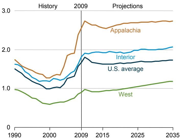
Figure 103. Average annual minemouth coal prices by region, 1990-2035 (2009 dollars per million Btu)
