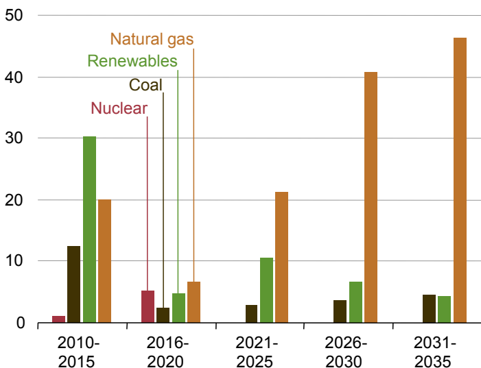
Figure 78. Electricity generation capacity additions by fuel type, 2010-2035 (gigawatts)
