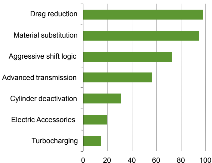
Figure 74. Market penetration of new technologies for light-duty vehicles, 2035 (percent)
