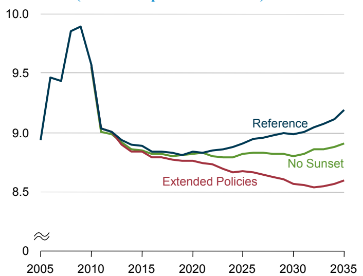
Figure 12. Average electricity prices in three cases, 2005-2035 (2009 cents per kilowatt-hour)
