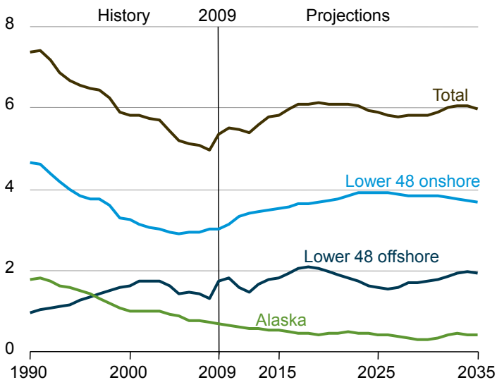
Figure 95. Domestic crude oil production by source, 1990-2035 (million barrels per day)
