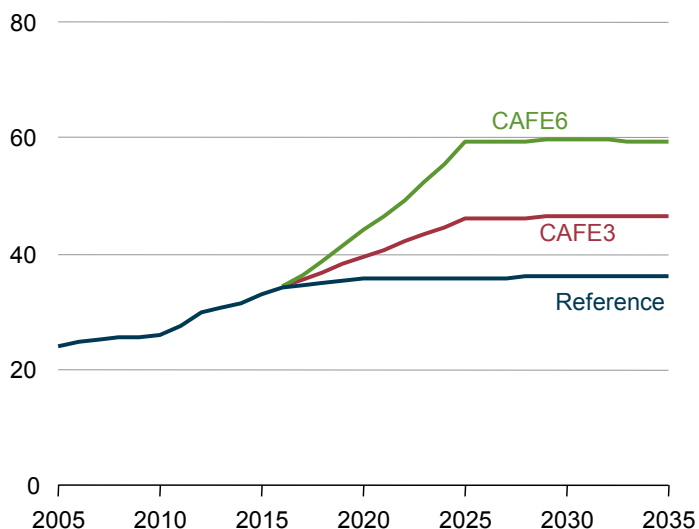
Figure 16. Combined CAFE standards for light-duty vehicles in three cases, 2005-2035 (miles per gallon)
