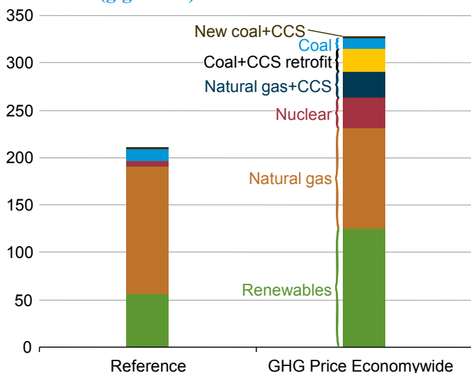
Figure 43. Cumulative capacity additions in the Reference and GHG Price Economywide cases, 2010-2035 (gigawatts)
