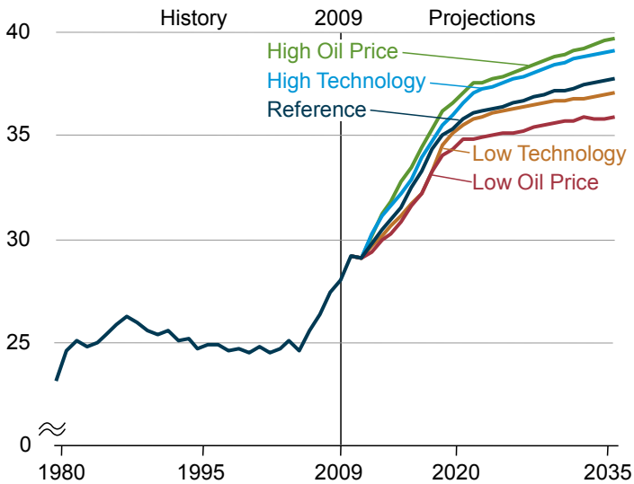
Figure 72. Average fuel economy of new light-duty vehicles in five cases, 1980-2035 (miles per gallon)
