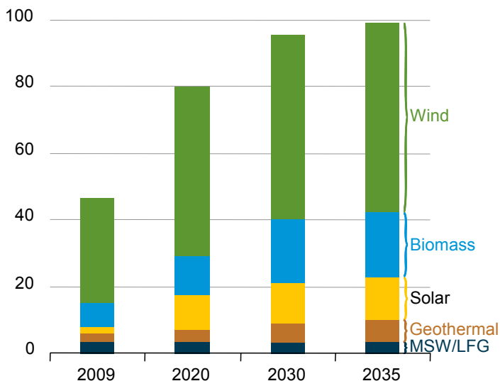
Figure 84. Nonhydropower renewable electricity generation capacity by source, 2009-2035 (gigawatts)
