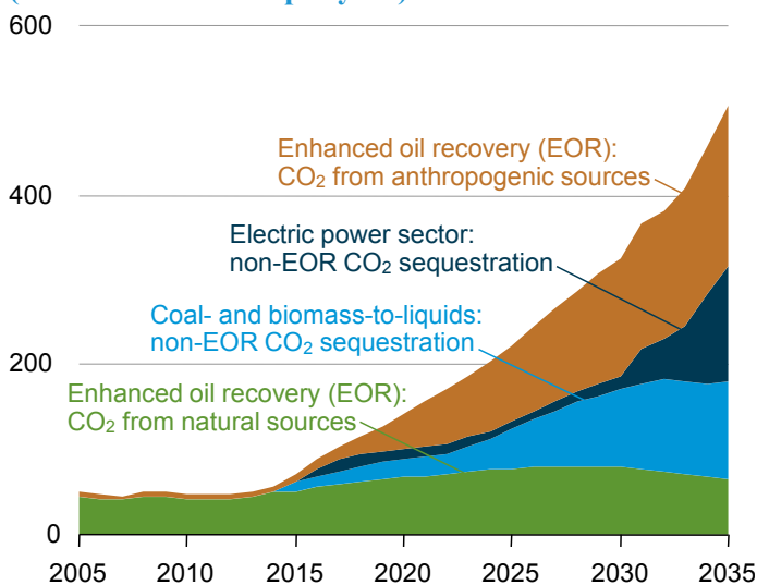
Figure 37. CO 2 injection volumes in the GHG Price Economywide case, 2005-2035 (million metric tons per year)
