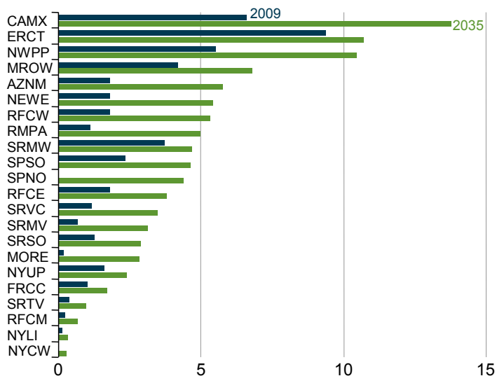
Figure 85. Regional growth in nonhydroelectric renewable electricity generation capacity, including end-use capacity, 2009-2035 (gigawatts)
